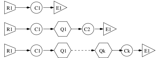
Figure 3: The Query Chain topology
